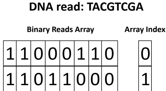
Figure 4.2: 2-bit encoding of TACGTCTGA.
